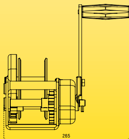
FRONT SPECIFICATIONS
