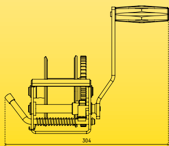
FRONT SPECIFICATIONS
