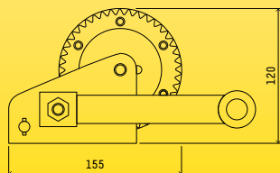
SIDE SPECIFICATIONS
