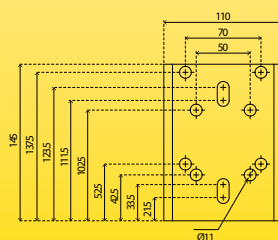
BASE SPECIFICATIONS
