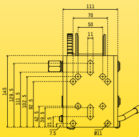
BASE SPECIFICATIONS
