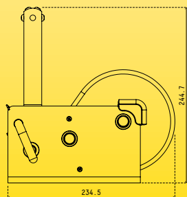
SIDE SPECIFICATIONS
