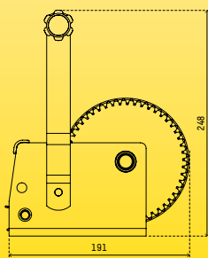
SIDE SPECIFICATIONS
