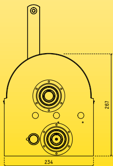
FRONT SPECIFICATIONS
