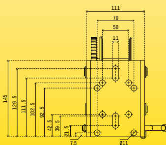
BASE SPECIFICATIONS
