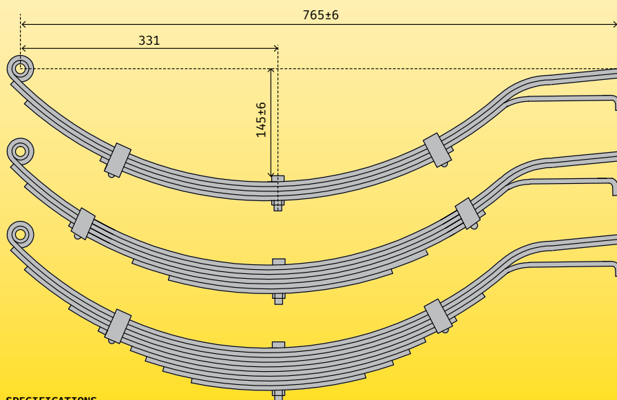
SPECIFICATIONS
