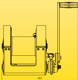
SIDE SPECIFICATIONS
