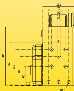
BASE SPECIFICATIONS
