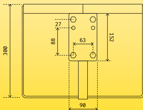
REAR/BOLTDOWN SPECIFICATIONS
