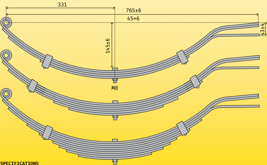
SPECIFICATIONS
