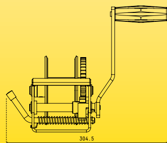
FRONT SPECIFICATIONS
