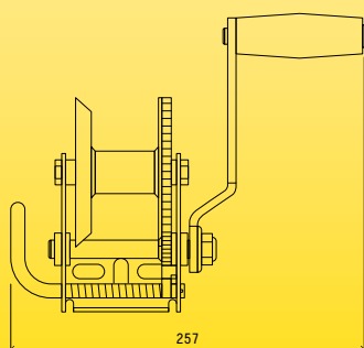
FRONT SPECIFICATIONS
