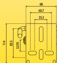
BASE SPECIFICATIONS
