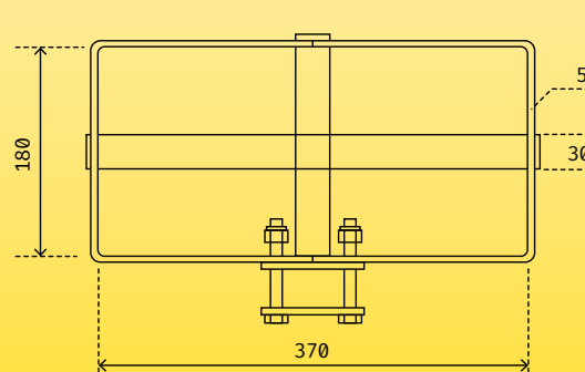
TOP/BASE SPECIFICATIONS
