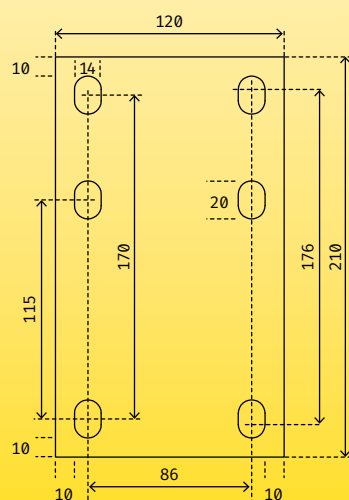
BOLT-DOWN SPECIFICATIONS
