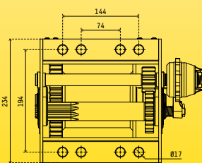
BASE SPECIFICATIONS
