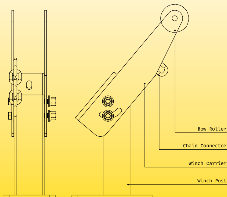
SPECIFICATIONS
