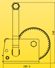
SIDE SPECIFICATIONS
