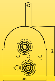
FRONT SPECIFICATIONS
