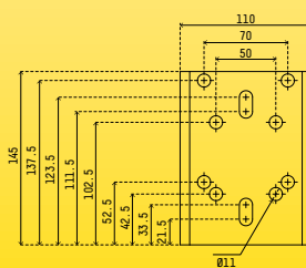
BASE SPECIFICATIONS
