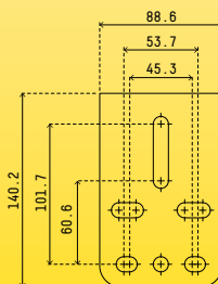
BASE SPECIFICATIONS
