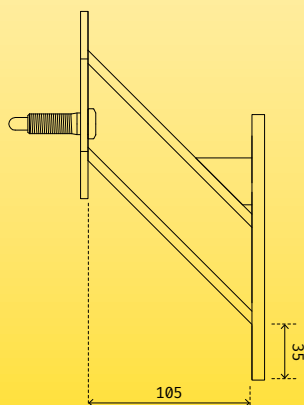
SIDE SPECIFICATIONS
