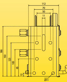
BASE SPECIFICATIONS
