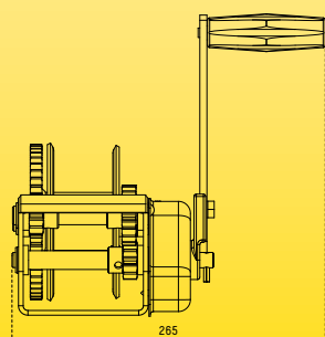
FRONT SPECIFICATIONS
