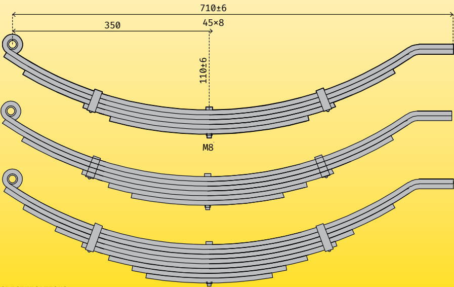
SPECIFICATIONS
