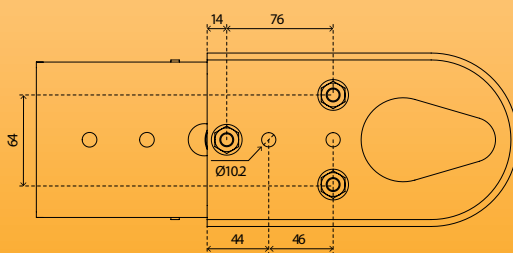
BASE SPECIFICATIONS
