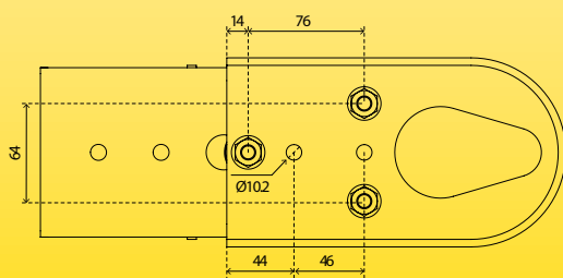
BASE SPECIFICATIONS
