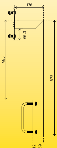
SIDE SPECIFICATIONS
