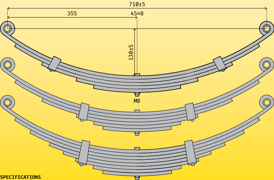
SPECIFICATIONS
