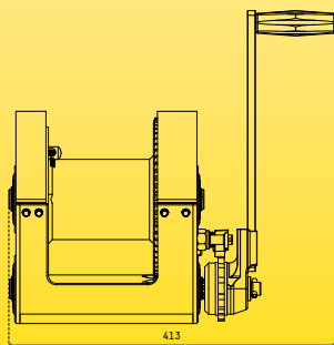
SIDE SPECIFICATIONS
