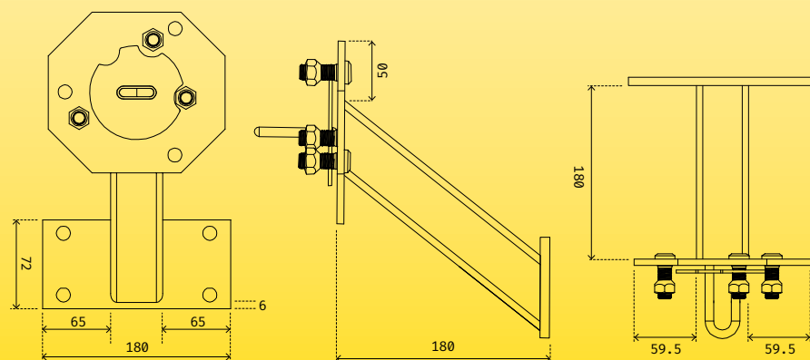
FRONT SPECIFICATIONS
